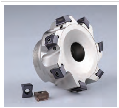
ASM90-LN09/LN13 square shoulder milling cutter with 4 cutting edge tangential inserts with helical edge profile. The reliable cutting edge can adopt increased fz by 30%, and also bring on higher metal removal rate and productivity.
